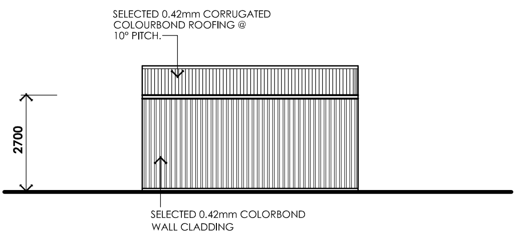
SIDE ELEVATION 1:100
