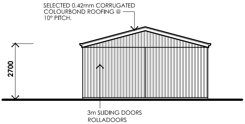
FRONT ELEVATION 1:100
