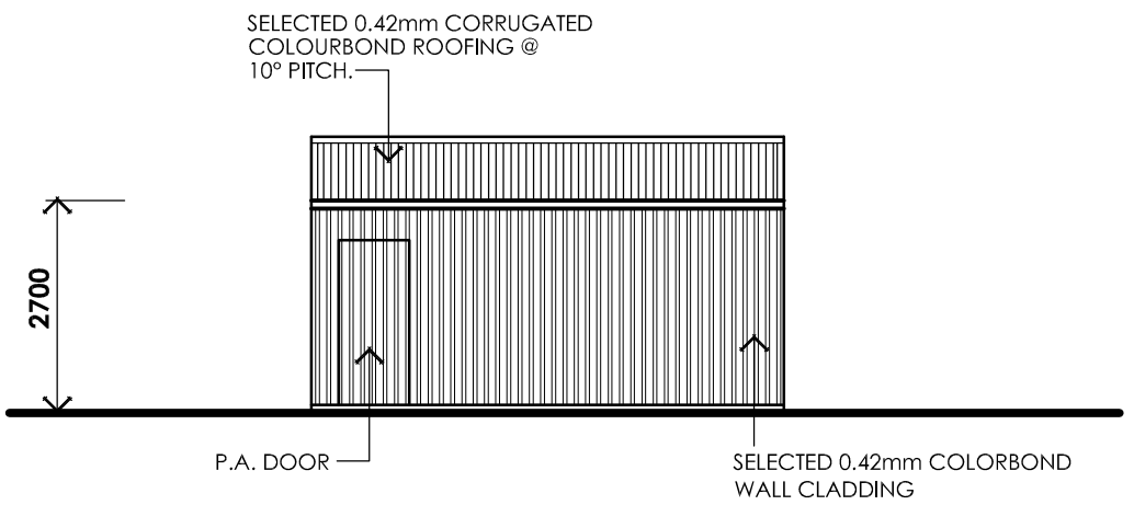
SIDE ELEVATION 1:100
